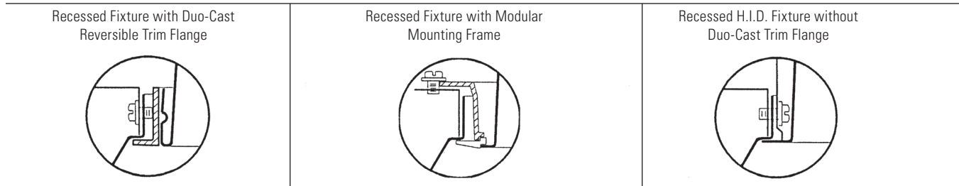
Detail of Attaching Fixture to Sloped Ceiling Adapter
