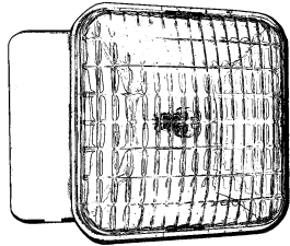
Backplate: 4.5" (11.4 cm) X 6.0" (15.2 cm) Single Head Depth: 4.0" (10.2 cm)
